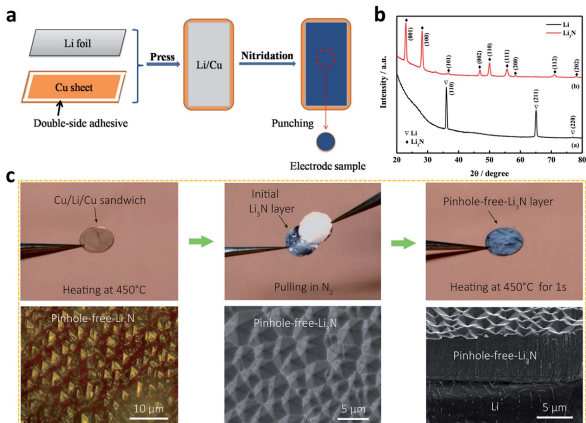
Fig. 3 Constructing artificial SEI layers on Li metal electrodes via chemical methods. (a) Preparation of a \text{Li}_3\text{N} film on an Li surface by utilizing the reaction between \text{N}_2 gas and Li metal; (b) characterization of the \text{Li}_3\text{N} film by X-ray diffraction (XRD); 72 reproduced with permission. Copyright 2015, Elsevier. (c) Preparation of a pinhole-free \text{Li}_3\text{N} layer to protect the Li metal electrode, and optical and scanning electron microscope (SEM) images of the pinhole-free \text{Li}_3\text{N} layer. 74 Reproduced with permission. Copyright 2018, American Chemical Society.
