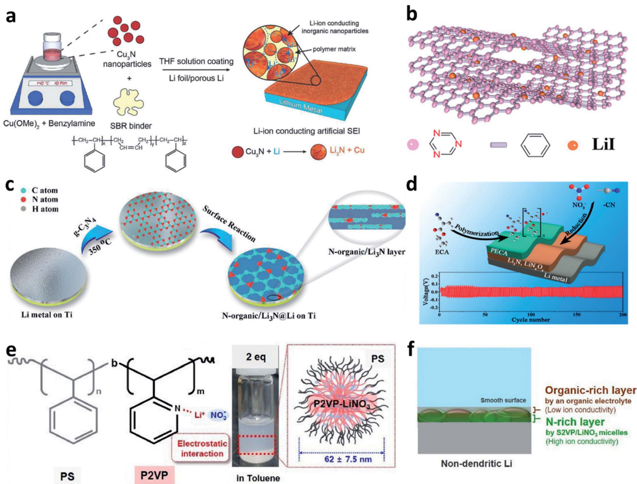
Fig. 4 Constructing nitrated organic-inorganic composite interfaces for Li metal electrodes. (a) Preparation of a \text{Cu}_3\text{N} -SBR interface on a Li metal electrode; 76 reproduced with permission. Copyright 2017, John Wiley and Sons. (b) Structural illustration of the CTF-LiI composite layer; 77 reproduced with permission. Copyright 2020, John Wiley and Sons. (c) Preparation of an N-organic/ \text{Li}_3\text{N} composite layer on a Li metal electrode; 78 reproduced with permission. Copyright 2020, John Wiley and Sons. (d) Schematic illustration of the preparation of a PECA- \text{Li}_3\text{N} / \text{LiNO}_3 dual protection layer for a Li metal electrode and the subsequent electrochemical performance. 79 Reproduced with permission. Copyright 2017, American Chemical Society. (e) Chemical structure, optical image, and schematic illustration of the \text{S}_2\text{VP}/\text{LiNO}_3 micelles; (f) schematic illustration of the multilayered structure formed on the surface of \text{S}_2\text{VP}/\text{LiNO}_3 -Li. 81 Reproduced with permission. Copyright 2021, Elsevier.
