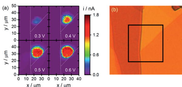
Fig. 6 Carrier confinement within more complex defect geometries. (a) CG-TC SECCM photocurrent images with the photoexcitation located near a triangular boundary within an n\text{-WSe}_2 nanosheet. (b) An optical transmission image of the same nanosheet, with the area interrogated via SECCM indicated. Experimental parameters were identical to those employed in Fig. 2.
