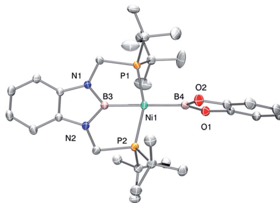
Fig. 1 Molecular structure of 3 (H atoms omitted for clarity). Thermal ellipsoids are represented at the 50% probability level. Selected bond distances (Å) and angles ( ^\circ ): \text{Ni}(1)\text{--B}(4) = 2.015(2) ; \text{Ni}(1)\text{--B}(3) = 1.942(2) ; \text{P}(1)\text{--Ni}(1)\text{--P}(2) = 157.74(3) ; \text{B}(3)\text{--Ni}(1)\text{--B}(4) = 175.0(1) .
