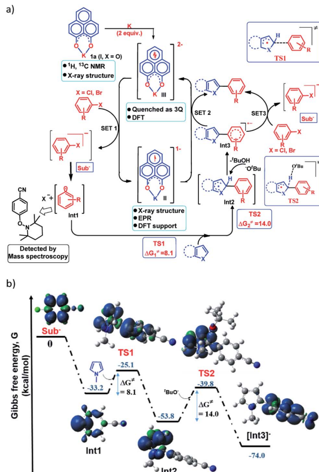
Fig. 4 (a) Proposed mechanistic cycle for the C–H arylation reaction by aryl halide activation; (b) reaction pathway by DFT calculations along with the geometry and spin density plot (α-spin in blue and β-spin in green color) of the reactive intermediates and transition states.
