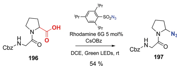
Scheme 49 Photocatalytic decarboxylation-azidation by Leonori et al. 137
