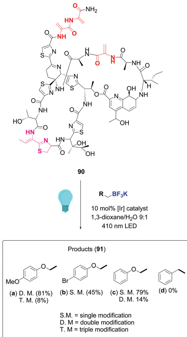
Scheme 23 Thiostrepton functionalization by Roelfs et al. 81
