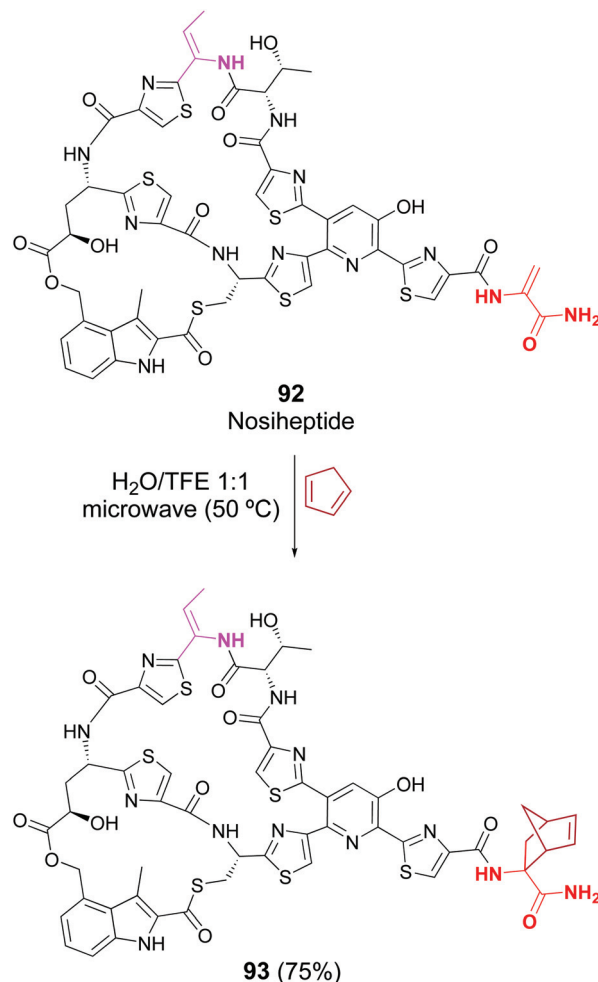
Scheme 24 Selective [2 + 4]-cycloaddition in nosiheptide by Roelfs et al. 83b
