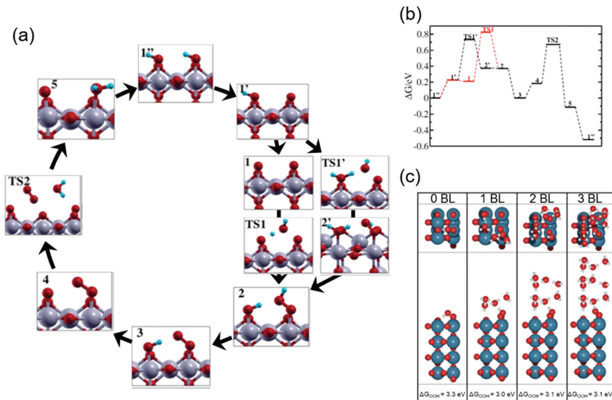
Fig. 3 Theoretical studies for H 2 O oxidation over iridium oxide. (a) Considered reaction pathways for the OER over the IrO 2 (110) surface; red balls are O; blue balls are H; silver balls are Ir. (b) Computed reaction free energy diagram at the constant potential of 1.36 V vs. normalized hydrogen electrode (NHE) at pH 0 (corresponding to 1.36 V vs. RHE at pH 0) corresponding to the mechanism shown in the panel (a). Reprinted with permission from ref. 46. Copyright (2017) American Chemical Society. (c) The most stable structure for the IrO 2 (110) surface with adsorbed *OOH at the coordinatively unsaturated metal sites (CUS), *O on the neighboring CUS, and *O at the bridge, together with varying numbers of water bilayers (BL); blue balls are Ir; red balls are O; white balls are H. Reprinted with permission from ref. 47. Copyright (2017) American Chemical Society.
