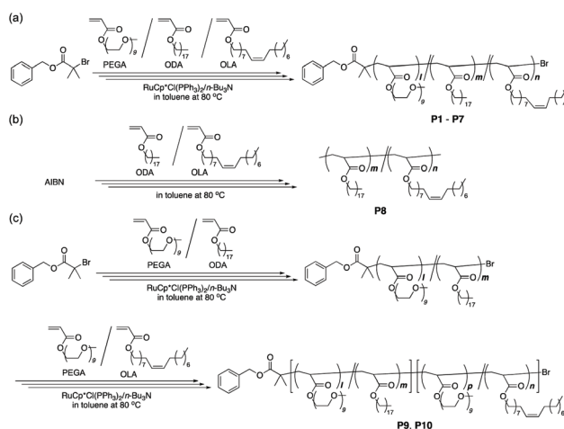
Scheme 1 Synthesis of (a) PEGA/ODA/OLA random terpolymers and PEGA/ODA or OLA random copolymers ( P1–P7 ), (b) an ODA/OLA random copolymer ( P8 ), and (c) PEGA/ODA-PEGA/OLA random block terpolymers ( P9 and P10 ) via living or free radical copolymerization.
