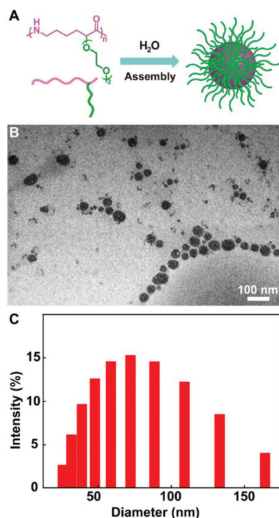
Fig. 8 Self-assembly of amphiphilic poly(OEGCL) into micelles. (A) Illustration on the formation of micelles. (B) TEM image of the micelle sample drop deposited from \text{H}_2\text{O} onto a carbon-coated copper grid; scale bar = 100 nm. (C) Size distribution of micelles measured by DLS. Reproduced from ref. 27 with permission from the American Chemical Society, copyright 2018.
