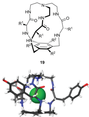
Fig. 12 General chemical structure of chloride receptors 19 based on pseudopeptidic tripodal cages (top) and crystal structure of compound 19a ( R^1 = \text{CH}_2\text{Ph}(4\text{-OH}) , R^2 = \text{Me} , bottom).
