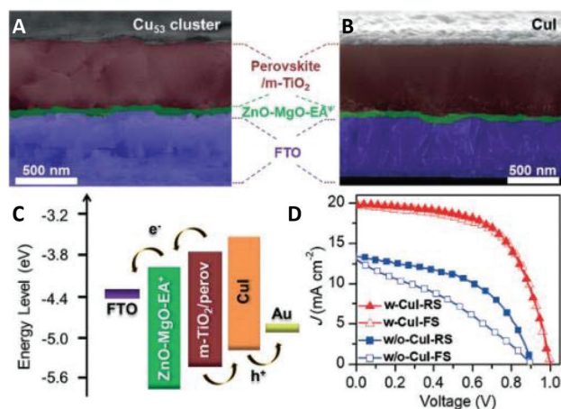
Fig. 38 Device structure and cross-sectional SEM image of (A) Cu 53 and (B) CuI on perovskite films. (C) Energy-level diagram of CuI-based perovskite solar cell (PSC). (D) Best J–V curves of devices with CuI (w-CuI) and without CuI (w/o-CuI). FS = forward scan, RS = reverse scan. Adapted with permission from ref. 194. Copyright 2019 Wiley-VCH Verlag GmbH & Co. KGaA, Weinheim.
