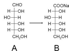
Scheme 2 Glucose oxidation to gluconic acid using metal NC catalysts. The reaction was conducted under \text{O}_2 atmosphere in \text{NaOH} solution kept at pH 9.5 in ref. 213. A = glucose, B = gluconic acid.
