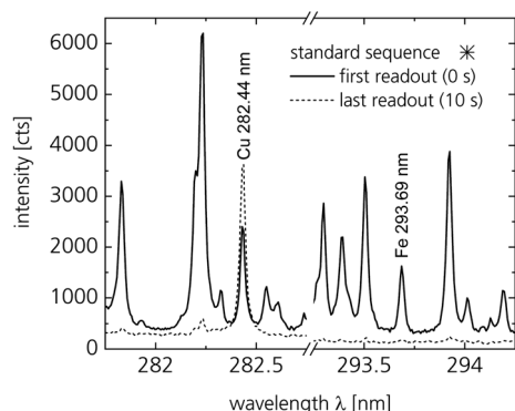
Fig. 3 Accumulated spectra of 15 plasma events in the wavelength interval of 281.8–294.3 nm measured in the standard sequence (the star-shaped data point is used here to indicate the relation to the data points shown in Fig. 4, right, for the standard sequence). Marked lines are used to determine the line ratio \tilde{Q}_{Fe} . The spectra were measured in the DPO mode after a preceding CM ablation phase.
