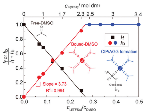
Fig. 17 Fraction of the integrated intensities of Raman peaks corresponding to free DMSO, I_f/(I_f + I_b) and bound DMSO, I_b/(I_f + I_b) in the LiTfSA/DMSO solutions. Reprinted with permission from ref. 38 Copyright 2017 American Chemical Society.
