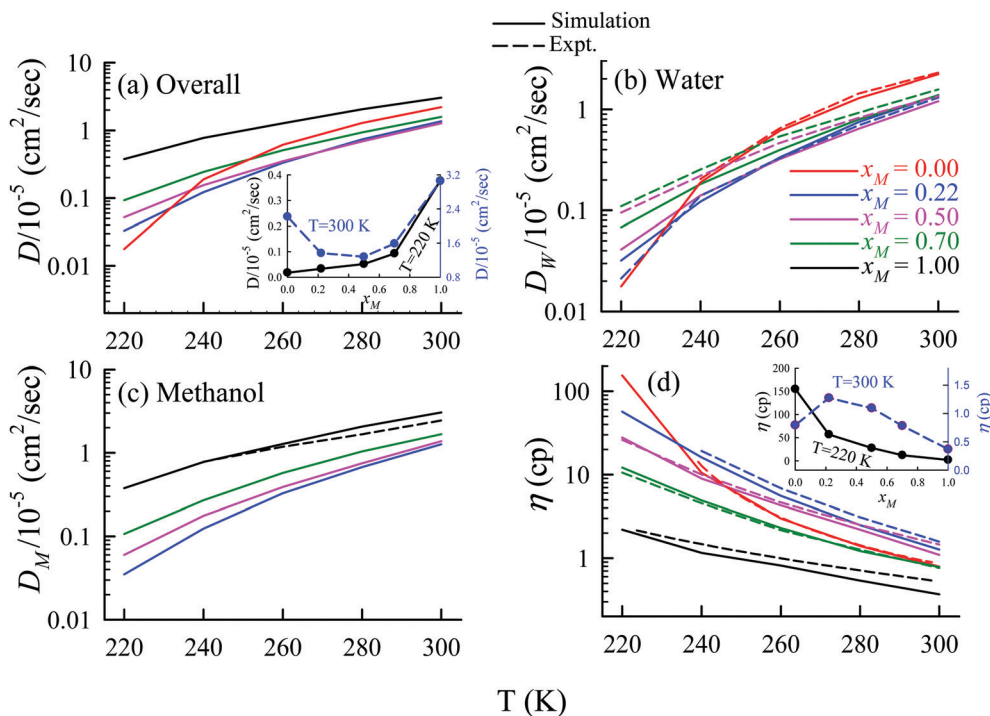
Fig. 12 Comparison between simulated (solid line) and experimental (dashed line) transport coefficients. (a) Temperature-dependent overall self-diffusion coefficient D for different systems. The inset shows the non-monotonic composition dependence of D at 300 K and monotonic composition dependence at 220 K. (b and c) Temperature-dependent diffusion coefficients of water ( D_W ) and methanol ( D_M ), respectively. (d) Temperature-dependent shear viscosity coefficient ( \eta ) for different systems. The inset of (d) shows the non-monotonic composition dependence of \eta at 300 K and monotonic composition dependence at 220 K. Reprinted with permission from ref. 66. Copyright (2020) American Chemical Society.
