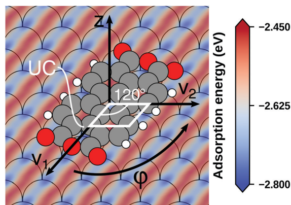
Fig. 21 Potential energy surface for the translation of a rigid PTCD molecule 2.9 \text{ Å} above the Ag(111) surface, calculated for a 6 \times 6 supercell using PBE+vdW surf , as obtained by Hörmann et al. 282 v_1 and v_2 denote the primitive lattice vectors of the substrate, z the adsorption height and \phi the rotation angle of the molecule relative to the substrate. The potential energy surface shows a minimum on the Ag-bridge site, a low-energy saddle point along v_1 and a high-energy saddle point along v_2 .
