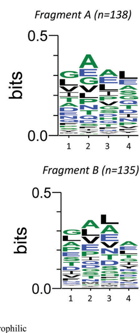
Fig. 9 (Generated using WebLogo): 47,48 (A) sequence Logos for peptides with a single modified cysteine exhibiting two-fold reduction in labeling segmented by “C” in the sequence (B) sequence Logos for peptides with a single modified cysteine that showed an increase in labeling segmented by “C” in the sequen.
