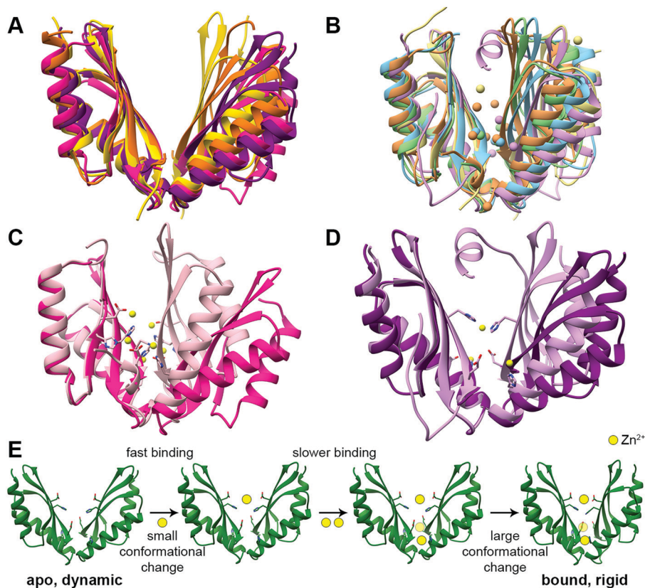
Fig. 2 The structures and suggested Zn^{2+} binding mechanism of the CTDs of CDF proteins. (A) Apo CTD structures of CzrB (PDB code: 3BYP, 41 pink), MamM (PDB code: 3W5X, 40 purple), MamB (PDB code: 5HO5, 43 yellow) and TM 0876 from Thermotoga maritima (PDB code: 2ZZT, 54 orange) overlapped onto each other. (B) Bound CTD structures of CzrB with Zn^{2+} (PDB code: 3BYR, 41 light pink), MamM with Cu^{2+} (PDB code: 6GP6, 53 light purple), MamB with Zn^{2+} (PDB code: 5HO1, 43 light yellow), EcYiiP with Zn^{2+} (PDB code: 3H90, 38 light green) and SoYiiP with Zn^{2+} (PDB code: 5VRF, 36 light blue) overlapped. In each structure, the DDMCs are presented as enlarged spheres in the proteins' colors. (C) The apo (dark pink) and Zn^{2+} -bound (light pink) structures of CzrB CTD and (D) the apo (dark purple) and Cu^{2+} -bound (light purple) structures of MamM CTD show the tighter conformation of the CTD that is achieved due to DDMC binding. The DDMCs are presented in yellow color and binding site residues are presented as sticks. (E) Zn^{2+} binding mechanism of MamM CTD (the model is adopted from Barber-Zucker et al. , 52 Zn^{2+} ions are presented as yellow spheres). Rapid Zn^{2+} binding (<1 microsecond) to the dynamic apo form's central site results in a minor conformational change but has an allosteric positive effect on the binding to the peripheral sites. Only slower (millisecond time scale) binding of two ions to the symmetrical sites causes a closure of the CTD to a tighter, rigid V-shape.
