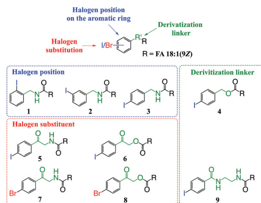
Fig. 1 Structural features of derivatives to be optimized for enhanced photofragmentation conversion at 266 nm. Structures 1 – 9 of derivatives conjugated to FA 18:1(9Z) (represented as R) used for structure–activity optimization.
