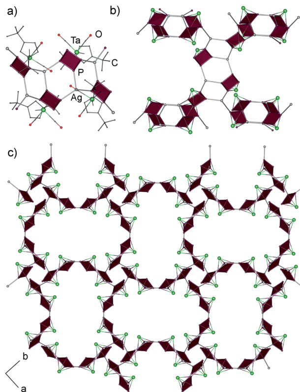
Fig. 3 (a) Repeating unit of 6 surrounded by four similar units (b) and (c) a section of the 3D coordination polymer in 6. \text{Cp}'' and carbonyl ligands as well as counter anions \text{SbF}_6^- are omitted for clarity.
