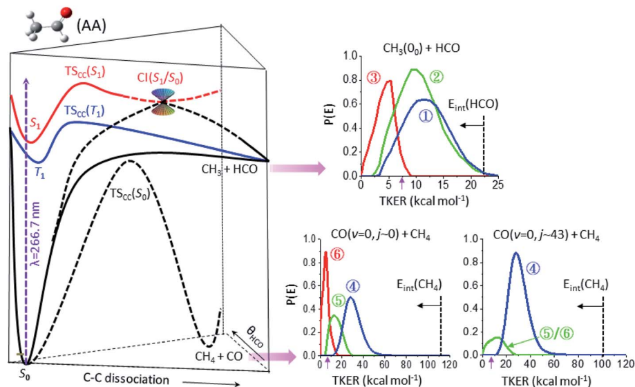
Fig. 3 The final product kinetic energy distributions and the potential energy surfaces that lead to their formations. (Left) Schematic of three potential energy surfaces of \text{CH}_3\text{CHO} (AA), S_0 (black), T_1 (blue), and S_1 (red), showing the correlation with the \text{CH}_3 + \text{HCO} and \text{CH}_4 + \text{CO} fragments. (Right) The final kinetic energy distributions ( \Delta t \rightarrow \infty ) of the individual components of three different product channels: top for \text{CH}_3(0_0) + \text{HCO} , lower-left for \text{CO}(v=0, j \sim 0) + \text{CH}_4 , and lower-right for \text{CO}(v=0, j \sim 43) + \text{CH}_4 . The color code is the same as that in Fig. 2c and the vertical dashed lines mark the energetic limits. By conservation of energy, the P(E) distribution can be regarded as a mirror image of the internal energy distribution of the co-fragments with the horizontal arrow indicating the increase of internal energy. The purple arrow near 7.4 kcal mol -1 marks the energetic limit for triple fragmentation.
