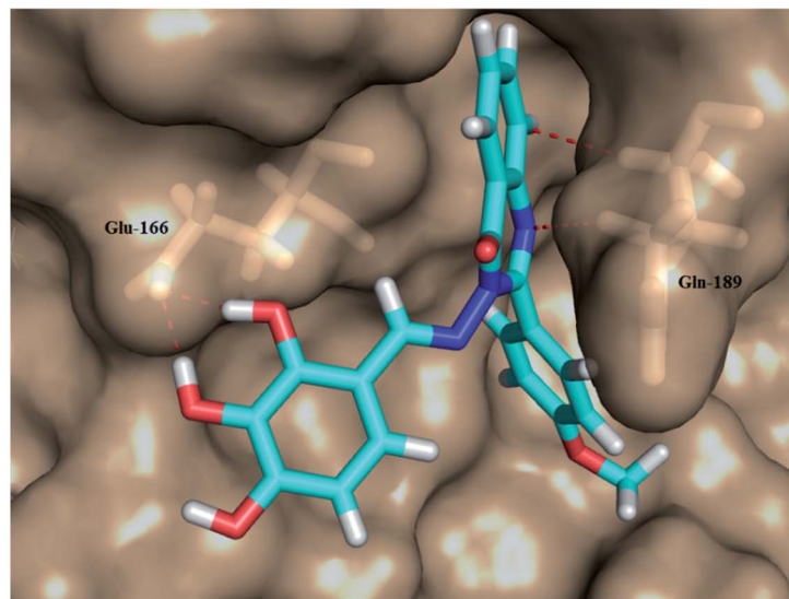
Fig. 7 (a) A 2D animated structure showing the binding interactions between compound 1c and M^{pro} and (b) a 3D representation showing the position of compound 1c within the cavity of M^{pro} .
