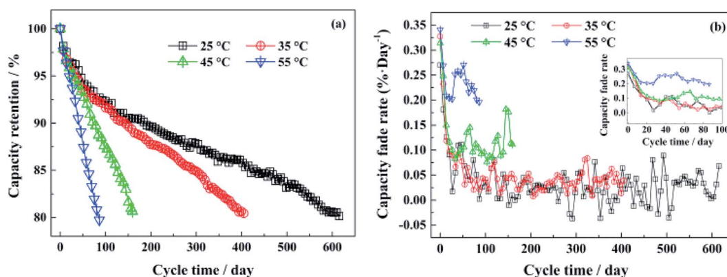
Fig. 10 (a) The capacity retentions of the \text{LiFePO}_4 /graphite full cells at different temperatures with continuous cycling days, (b) the capacity fade rate at each test temperature during cycling. 113
