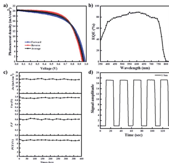
Fig. 8 (a) The hysteresis of the J – V curves in both scan directions under AM 1.5 irradiation (100 mW cm −2 ), (b) EQE spectra, (c) stability, and (d) photoswitching phenomenon for the most efficient PHJ PrSCs fabricated using dip-coating deposition approach on the thin ZnO/c-TiO 2 bilayer ETL under two SDC cycles.
