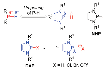
Fig. 1 1,3,2-Diazaphospholenes exhibit an Umpolung of the P–H bond.
