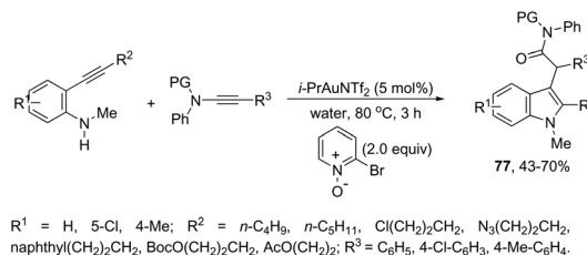
Scheme 65
