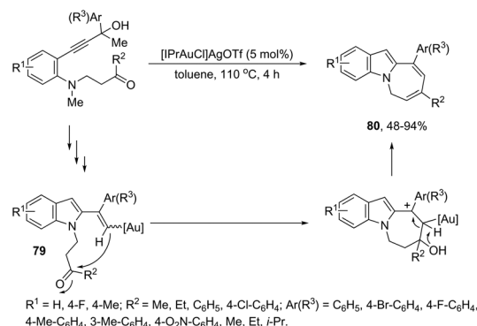
Scheme 67
