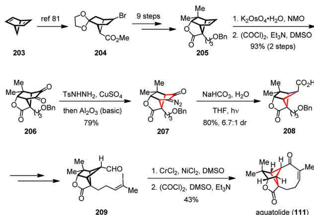
Scheme 28 Wolff rearrangement in the total synthesis of aquatolide.
