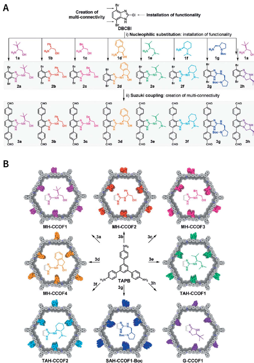
Fig. 42 Construction of combinatorial library of COFs. (A) Divergent synthesis of chiral monomers from DBCBI by nucleophilic substitution and Suzuki coupling. (B) Divergent synthesis of COFs by imine formation. Adapted with permission. 263 Copyright 2019, Wiley-VCH Verlag GmbH & Co. KGaA, Weinheim.
