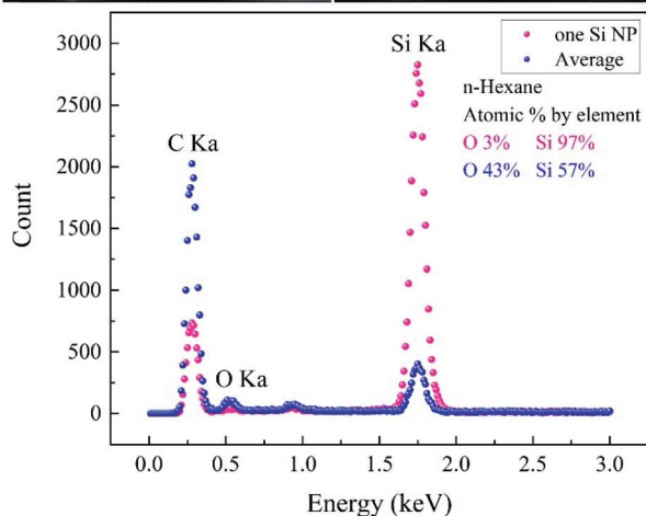
Fig. 7 The femtosecond laser-synthesized Si nanoparticles in n -hexane. ( N = 1000 , F = 10.46 \text{ J cm}^{-2} ). The TEM bright-field image, SAED pattern (upper right) and dark-field images related to different diffracted electron beams along the 1 st and 2 nd ring. The EDX spectrum from several small Si NPs and one Si NP.
