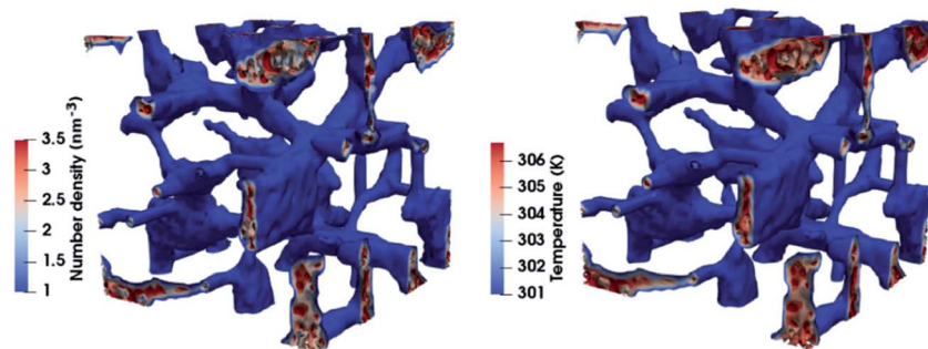
Fig. 6 Isodensity surfaces of CNTs (9% in weight) in linear polymer assembled morphology (left panel) and temperatures isosurfaces (right panel) computed after the application of potential difference on that configuration. The employed grid size is 2.05 nm.
