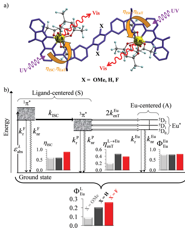
Fig. 6 (a) Molecular structures and (b) simplified Jablonski diagram for [(\text{hfac})_3\text{Eu}(\text{L})\text{Eu}(\text{L})_2]_3 showing the indirect ligand-centred triplet-mediated sensitization mechanism of the two Eu 3+ activators. The photophysical processes are described by first-order rate constants: k_r^F = ligand fluorescence, k_{nr}^F = ligand internal non-radiative conversion, k_r^P = ligand phosphorescence, k_{nr}^P = non-radiative relaxation from the ligand triplet state, k_r^{Eu} = emission of Eu*, k_{nr}^{Eu} = nonradiative decay of Eu*, k_{ISC} = ligand intersystem crossing, and k_{en.tr.}^{Eu} = ligand-to-metal energy transfer. Efficiencies of intersystem crossing ( \eta_{ISC} ), of energy transfer ( \eta_{en.tr.}^{Eu} ), of intrinsic quantum yield ( \Phi_{Eu}^{Eu} ), and global quantum yield ( \Phi_{Eu}^{Eu} ) characterize the antenna effect (solid-state, 293 K). Adapted from ref. 17b.
