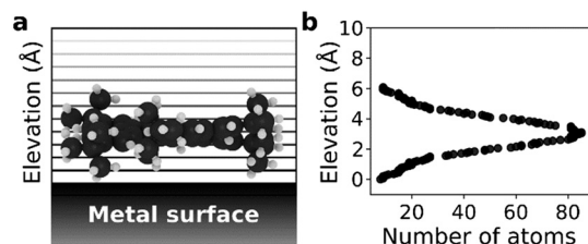
Fig. 4 Elevation weighted density calculation for HtBDC: (a) starting from the bottom most part of the molecule, number of atoms are counted with 0.05 Å discrete steps and using a cut-off radius of 1 Å (b) for each step number of atoms in proximity of that elevation are plotted.
