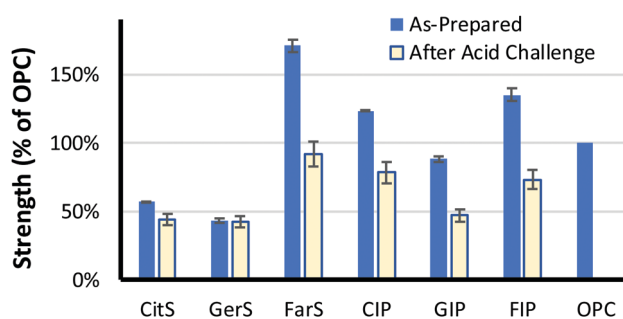
Fig. 4 Compressive strength of terpenoid–sulfur composites ( CitS , GerS , and FarS ), ordinary Portland cement (OPC) and composite-infused cement ( CIP , GIP , and FIP ) measures before (blue bars) and after (yellow bars) being submerged in 0.5 M H 2 SO 4 for 24 h. OPC deteriorates after acid challenge so its post-acid strength could not be determined. Each measured value is an average of three trials, and the error bars represent the standard deviation of the three runs.
