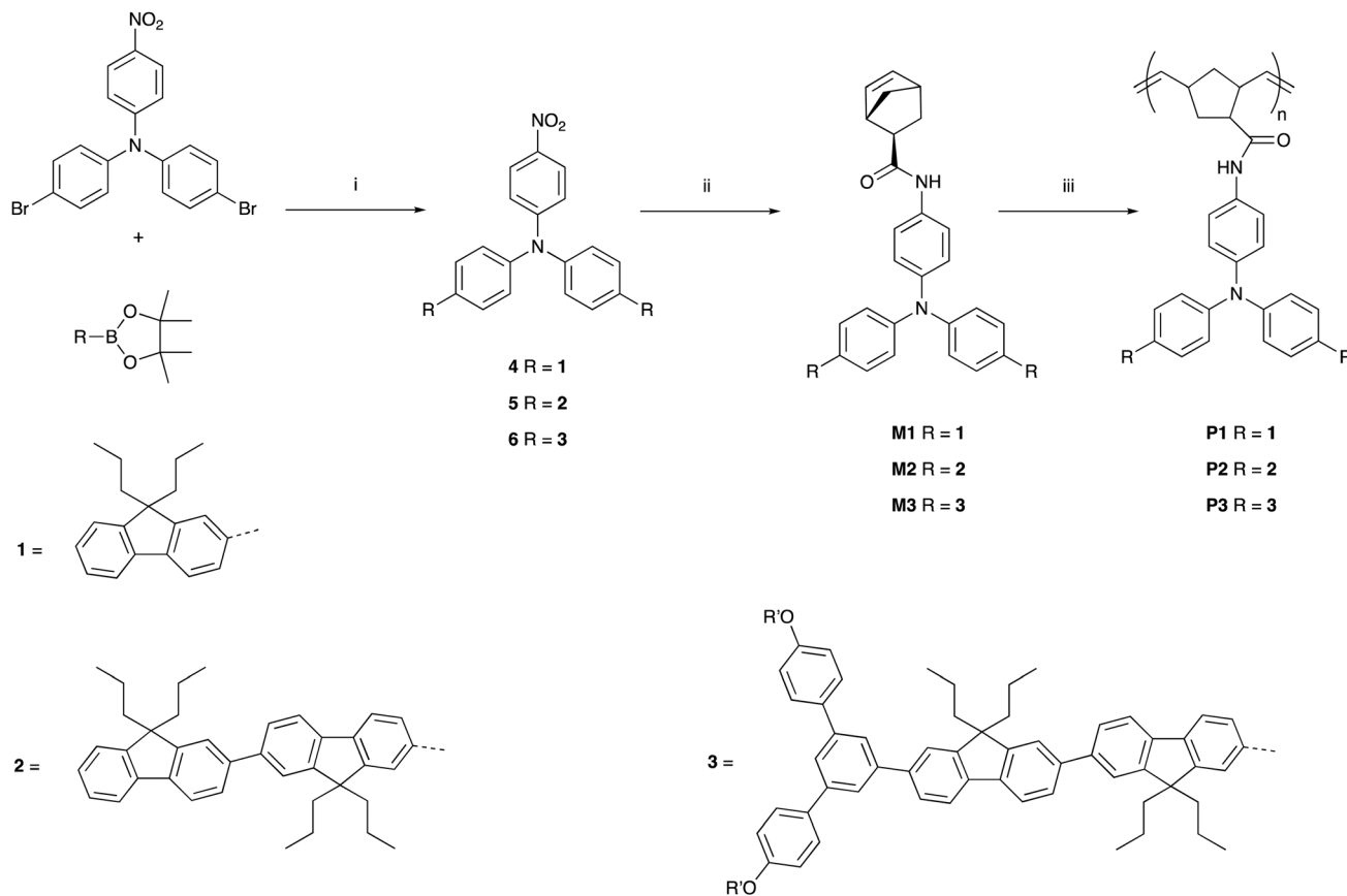
Scheme 1 Reactions and conditions (i) \text{Pd(PPh}_3)_4 , aq. \text{K}_2\text{CO}_3 , PhMe, Ar, heat; (ii) \text{Pd/C} (10% w/w), \text{H}_2 , \text{CHCl}_3 , EtOH, r.t. then (1 S ,4 R )-bicyclo[2.2.1]hepta-2,5-diene-2-carboxylic acid (97% exo ), DCC, DMAP, DCM, r.t.; (iii) Grubbs third generation catalyst (1 mol% or 5 mol%), THF, r.t. R' = 2-ethylhexyl.
