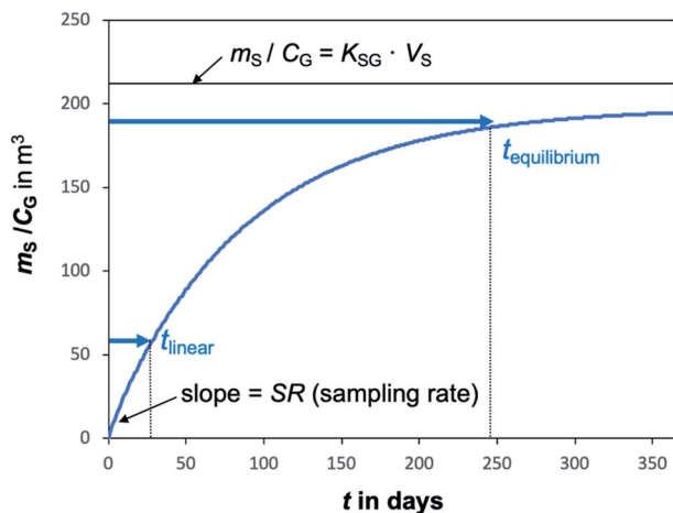
Fig. 2 Generic illustration of the uptake of an SVOC in a passive air sampler, showing the increase in the sorbed amount m_s divided by the atmospheric concentration C_G as a function of deployment time t . The time period of linear uptake t_{\text{linear}} and the time to equilibrium t_{\text{equilibrium}} are important characteristics of a passive sampler. The displayed curve was calculated with PAS-SIM 21 for a compound with \log K_{\text{SG}} of 6 in a PUF-PAS and an SR of 3.2 m 3 per day. A t_{\text{equilibrium}} of 246 days is based on C_s/K_{\text{SG}} > 0.90C_G and a t_{\text{linear}} of 24 days is based on C_s/K_{\text{SG}} < 0.25C_G . See Section F.5 for more information on the PAS-SIM model.
