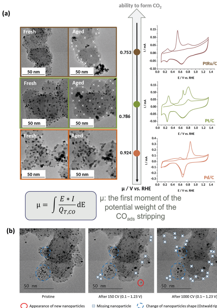
Fig. 11 (a) IL-TEM micrographs pre-AST and post-AST and \text{CO}_{\text{ads}} stripping voltammograms recorded at v = 20 \text{ mV s}^{-1} in 0.1 M NaOH on 10 wt% PtRu/C (brown), 10 wt% Pt/C (green), and 10 wt% Pd/C (orange). The extent of nanoparticles detachment is correlated with the average \text{CO}_{\text{ad}} stripping potential (first moment of the potential weight of the \text{CO}_{\text{ads}} stripping). (b) Representative IL-TEM micrographs of Pt/C nanoparticles before (pristine) and after 150 or 1000 CV cycles performed at v = 100 \text{ mV s}^{-1} between 0.1 and 1.23 V vs. RHE in interface with an anion-exchange membrane in the dry cell at T = 25 \text{ }^\circ\text{C} . The markers are not comprehensive and just illustrate the main degradation mechanisms at stake during the potential cycling procedure. Reproduced from ref. 242 with permission from the American Chemical Society.
