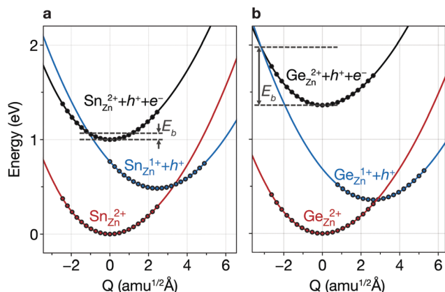
Fig. 5 Configuration coordinate diagram for carrier capture. Potential energy surfaces for the vibrations of \text{Sn}_{\text{Zn}}^{(2+/+)} in \text{Cu}_2\text{ZnSnSe}_4 (a) and \text{Ge}_{\text{Zn}}^{(2+/+)} in \text{Cu}_2\text{ZnGeSe}_4 (b). The solid circle represents the relative formation energy calculated using DFT, and the line is a spline fit. E_b represents the electron-capture barrier.
