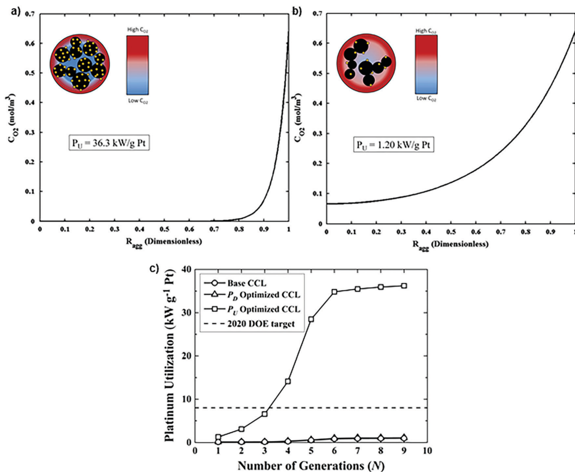
Fig. 19 (a) Dissolved oxygen concentration in a single agglomerate in a catalyst layer with m_{Pt} = 0.40 mg cm⁻², as a function of the dimensionless radial coordinate in an aggregate, r_{agg} . Cell operating at 0.40 V. (b) Dissolved oxygen concentration in a single agglomerate in a catalyst layer with an ultra-low platinum loading, m_{Pt} = 0.010 mg cm⁻². Cell operating at 0.40 V. (c) Effect of the number of fractal branching generations on platinum utilization ( P_U ) for the base and optimized CCL microstructures. The operating conditions are anode and cathode stoichiometry ratios of 1.5 and 2 respectively, r_{agg} = 100 nm, and 100% RH. Fig. 20(a and b) were reprinted with permission from ref. 351. Copyright 2013 Elsevier.
