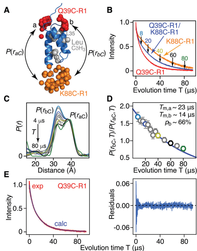
Fig. 2 Phase memory relation time ( T_{\text{m}} ) filtering for [Leu-CH 3 / 2 H] AviTag-Protein A (Q39C-R1/K88C-R1) in an otherwise perdeuterated background. (A) Ribbon diagram of the protein A core domain 22 (blue) with the oxygen atoms of the nitroxide spin label ensembles (generated using the rotamer library program MMM) colored in red (Q39C-R1) and orange (K88C-R1), and the leucine methyl groups in grey. The two distances between K88C-R1 and the two conformer populations ( a and b ) of Q39C-R1 are indicated. (B) Hahn spin-echo curves for [Leu-CH 3 / 2 H] AviTag-Protein A, spin-labeled at Q39C-R1/K88C-R1 (blue), Q39C-R1 (red) and K88C-R1 (orange). (C) P(r) distributions for [Leu-CH 3 / 2 H] AviTag-Protein A (Q39C-R1/K88C-R1) obtained from the DEER echo curves using DeerAnalysis 24 with Tikhonov regularization at evolution times T (= 2\tau_2) ranging from 8 to 80 μs. The color coding corresponds to that of the experimental points in panel D. The P(r) distributions are normalized with regard to the a peak at 38 Å. The DEER pulse scheme is shown in Fig. S1B (ESI † ), and the raw and background-corrected DEER echo curves are shown in Fig. S3 (ESI † ). Results of global best-fitting eqn (1) and (2) to the experimental evolution time T (= 2\tau_2) dependence of (D) the peak intensity ratio, P(r_{\text{bc}}, T)/P(r_{\text{ac}}, T) , in the P(r) distributions for [Leu-CH 3 / 2 H] AviTag-Protein A (Q39C-R1/K88C-R1) and (E) the Hahn echo curve for [Leu-CH 3 / 2 H] AviTag-Protein A (Q39C-R1) (left panel). The experimental ratios of the b to a peak intensities, P(r_{\text{bc}}, T)/P(r_{\text{ac}}, T) , are obtained from the integrated intensities of two Gaussians fitted to the bimodal P(r) distributions. The experimental data and best-fits are displayed by the circles and blue line, respectively in (D) and by the red and blue curves, respectively, in (E). Normalization in (E) was carried out by dividing the experimental and calculated curves by the optimized value of the sum of the two scale factors ( \lambda_1 + \lambda_2 ). The right panel in (E) is a plot of the distribution of residuals between experimental and calculated Hahn echo curves. The corresponding P(r) distributions and best fits obtained using DeerAnalysis with validated Tikhonov regularization, 24 the program DD with a sum of two Gaussians, 25 the program WavPDS (to filter out noise) 26 followed by Tikhonov regularization, 24 and WavPDS followed by SVD 26–28 are shown in Fig. S4–S7 (ESI † ), respectively.
