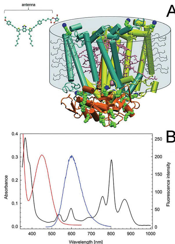
Fig. 9 (A) Crystallographic structure of the Rhodospira rubra R26 reaction center. The ubiquinone-10 molecules (Q A , Q B ), two bacterio-pheophytins, and four bacteriochlorophylls are in pink. Lysines are van der Waals green spheres. The terminal N 2 lysine targets of bioconjugation are in blue. The detergent toroid surrounding the hydrophobic portion of the protein is shown as a grey cylinder, including the detergent molecules (not to scale). The structure of the activated organic fluorophore antenna is shown in the upper left corner (C, cyan; N, blue; O, red; and S, yellow). The antenna and the RC structures are to scale. (B) Absorption spectra of the RC (black) and the artificial antenna (red). Fluorescence spectrum of the antenna (blue). Adapted with permission from F. Milano, R. R. Tangorra, O. Hassan Omar, R. Ragni, A. Operamolla, A. Agostiano, G. M. Farinola and M. Trotta, Enhancing the Light Harvesting Capability of a Photosynthetic Reaction Center by a Tailored Molecular Fluorophore, Angew. Chem., Int. Ed. , 2012, 51 , 11019–11023. Copyright 2012 Wiley-VCH Verlag GmbH & Co. KGaA.
