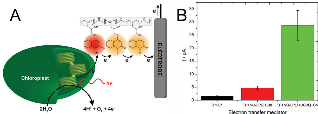
Fig. 7 (A) Artificial PEET process through the naphthoquinone-based redox polymer that harvests photoexcited electrons from intact chloroplast and shuttles them to the electrode surface. (B) Comparison of photocurrent generation from chloroplasts in direct electron transfer condition (TP + Chl, black), in the presence of the naphthoquinone redox polymer (TP + NQ-LPEI + Chl, red), and in the presence of both the redox polymer and diffusible dichloro benzoquinone (TP + NQ-LPEI + DCBQ + Chl, green). Adapted with permission from K. Hasan, R. D. Milton, M. Grattieri, T. Wang, M. Stephanz and S. D. Minter, Photobioelectrocatalysis of Intact Chloroplasts for Solar Energy Conversion, ACS Catal. , 2017, 7 , 2257–2265. Copyright 2017 American Chemical Society. 98
