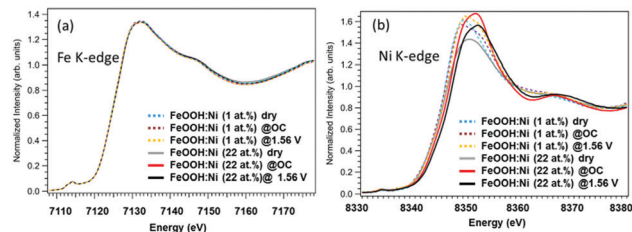
Fig. 2 (a) Fe and (b) Ni XANES spectra of 1% Ni ( \beta -FeOOH:Ni) and 22% Ni ( \beta -FeOOH:Ni surface-decorated with Ni(OH) 2 ) acquired under dry, OC potential and OER potential (+1.56 V) conditions.
