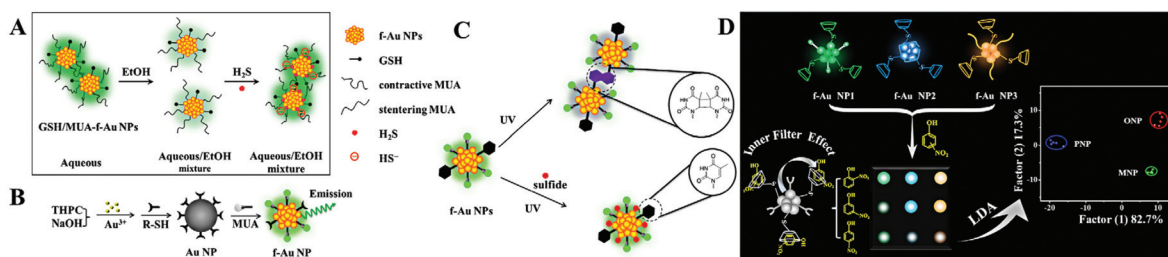
Fig. 4 (A) Schematic illustration of the H_2S detection principle using GSH/MUA-f-Au NP nanoprobe. Reprinted with permission from ref. 51. Copyright 2020, Springer. (B) Illustration of the synthetic route toward the preparation of dual-ligand protected f-Au NPs. Reprinted with permission from ref. 52. Copyright 2011, Royal Society of Chemistry. (C) Schematic principle of dual-ligand stabilized f-Au NPs for H_2S sensing. Reprinted with permission from ref. 53. Copyright 2013, Royal Society of Chemistry. (D) Illustration of f-Au NP array-based discrimination of nitrophenol isomers by integrating host-guest interaction and inner filter effect. Reprinted with permission from ref. 55. Copyright 2018, American Chemical Society.
