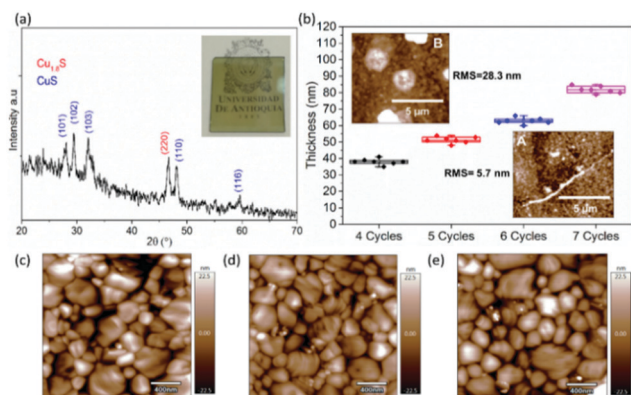
Fig. 15 Morphology of \text{Cu}_2\text{S} films and the perovskite. (a) XRD pattern revealing covellite and digenite phases with the inset showing the image of a typical \text{Cu}_2\text{S} electrode on a glass substrate; (b) dependence of the film thickness and roughness on the deposition cycles. Inset A: AFM image of a 4 cycles film (black symbols). Inset B: AFM image of a 7 cycles film (magenta symbols). AFM topography of the perovskite surface grown on (c) ITO; (d) 4 cycles \text{Cu}_2\text{S} ; and (e) 7 cycles \text{Cu}_2\text{S} . 118
