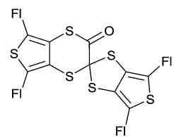
Fl = fluorene or oligofluorene
