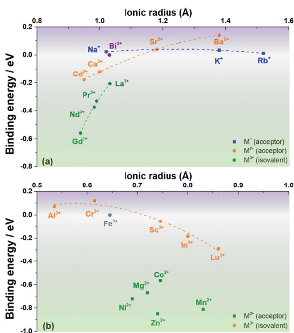
Fig. 2 Binding energies of a cation substituent-oxygen vacancy associate as a function of ionic radius for cations that prefer (a) the Bi site and (b) the Fe site of rhombohedral BiFeO 3 .
