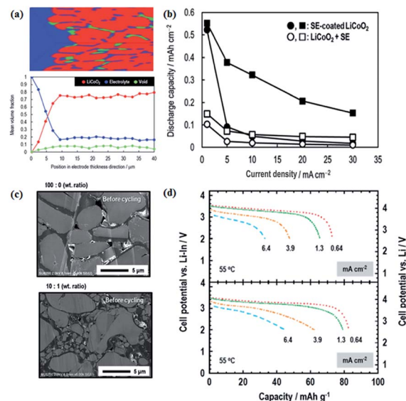
Fig. 12 (a) Volume fractions of respective materials along the electrode thickness; (b) electrochemical performance of S-SE-coated \text{LiCoO}_2 and \text{LiCoO}_2 + S-SE; (c) S-SE-coated \text{LiCoO}_2 particles with different grain sizes; (d) electrochemical performances of different cathode compositions. Reproduced with permission. 109 Copyright© 2017, Royal Society of Chemistry.
