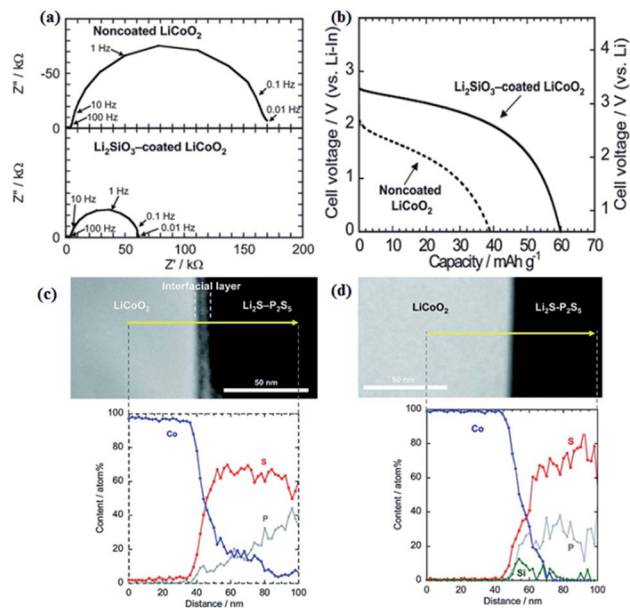
Fig. 11 (a) Impedance profiles of the all-solid-state cells In/ \text{Li}_2\text{S} - \text{P}_2\text{S}_5 with solid electrolyte non-coated and \text{Li}_2\text{SiO}_3 -coated \text{LiCoO}_2 at -30^\circ\text{C} after charging to 3.6 V vs. Li-In. (b) Discharge curves of the all-solid state cells under the current density of 0.064\text{ mA cm}^{-2} at 30^\circ\text{C} . (c) Cross-sectional HAADF-STEM image of \text{LiCoO}_2 electrode/ \text{Li}_2\text{S} - \text{P}_2\text{S}_5 solid electrolyte interface after initial charging and cross-sectional EDX line profiles for Co, P, and S elements. (d) Cross-sectional HAADF-STEM image of the \text{Li}_2\text{SiO}_3 -coated \text{LiCoO}_2 / \text{Li}_2\text{S} - \text{P}_2\text{S}_5 interface after initial charging and cross-sectional EDX line profiles for Co, P, S, and Si elements. 99,108 Reproduced with permission. Copyright© (2009, 2010), American Chemical Society.
