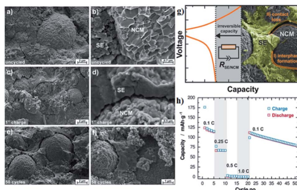
Fig. 13 (a and b) Scanning electron micrographs of the cathode composite of NCM811 and \beta\text{-Li}_3\text{PS}_4 as prepared in a solid-state cell but without the application of current or potential. (c and d) SEMs of a \text{Li-In}|\beta\text{-Li}_3\text{PS}_4|\text{NCM-811} batteries after single charging to 4.3 V vs. Li/Li + at 0.1 C. (e and f) SEMs of a given cell after 50 full battery cycles in the discharged state. (g) Schematic diagram of performance degradation mechanism in all-solid-state batteries. (h) Rate test and long-term cyclability for the all-solid-state batteries. Reproduced with permission. 116 Copyright© 2017, American Chemical Society.
