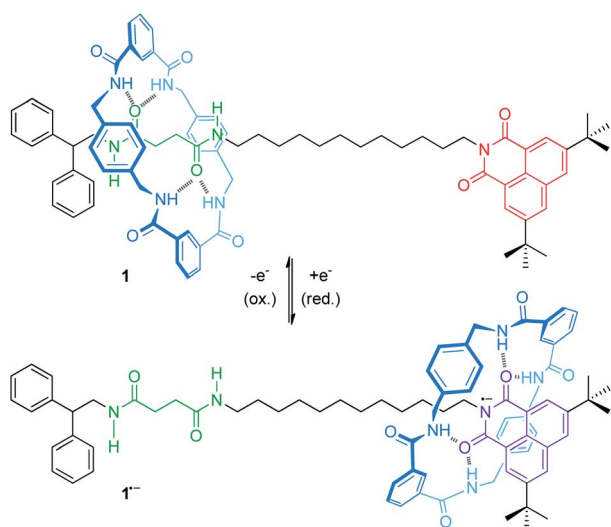
Fig. 2 Electrochemically switchable molecular shuttle 1 . In the neutral state, the tetralactam wheel preferably encircles the diamide station. One-electron reduction to the 1^{\cdot-} state moves the wheel to the naphthalimide radical anion site.
