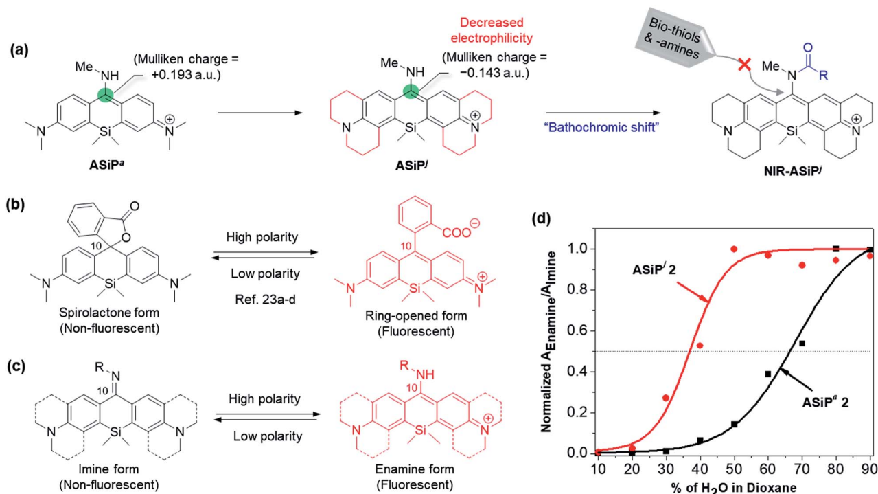
Fig. 3 (a) Far-red emitting julolidine-derived amino-Si-pyrone dyes (ASiP j ) and their NIR-emitting derivatives (NIR-ASiP j ) that are stable inside cells. The corresponding Mulliken charges at C-10 of ASiP a and ASiP j are shown in atomic unit (a.u.). Structural changes of (b) SiR and (c) ASiP dyes depending on the polarity of the medium. (d) Changes of the normalized absorbance ratio of the enamine form (fluorescent) to the imine form (non-fluorescent) depending on the medium polarity (increasing water content in 1,4-dioxane), compared for ASiP a 2 and ASiP j 2.
