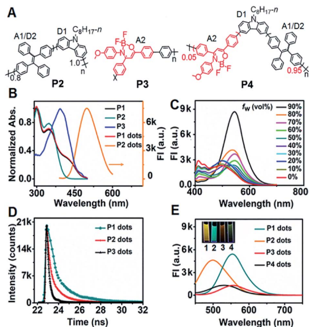
Fig. 1 (A) Structural formulae of P2 – P4 . (B) UV-vis absorbance of P1 – P3 in THF and P1 dots in H 2 O, and the FL spectrum of P2 dots in H 2 O at a \lambda_{\text{ex}} of 370 nm. (C) FL spectra of P1 in THF–H 2 O mixtures with different contents of H 2 O at a \lambda_{\text{ex}} of 370 nm. (D) FL lifetimes of P1 – P3 dots in H 2 O at a \lambda_{\text{ex}} of 374 nm. (E) FL spectra of 10 \mu\text{g mL}^{-1} P1 dots, 50 \mu\text{g mL}^{-1} P2 dots, 100 \mu\text{g mL}^{-1} P3 dots, and 50 \mu\text{g mL}^{-1} P4 dots at a \lambda_{\text{ex}} of 370 nm. Inset: FL photos of P1 – P4 dots.
