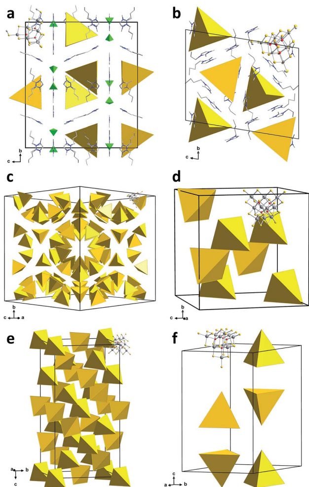
Fig. 2 Sections of the crystal structures of 1a (a), 1b (b), 1c (c), 1d (d), 1e (e) and 1f (f). [\text{Sn}_{10}\text{S}_{16}\text{O}_4(\text{S-Me})_4]^{4-} anions, except one, are shown as yellow tetrahedra; green tetrahedra represent [\text{BF}_4]^- anions. Counterions are shown in wire representation. Color code: grey – Sn, yellow – S, red – O, light grey – C, blue – N.
