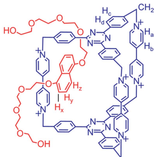
\text{BH4EN} \cdot \text{AzaEx}^2\text{Cage}^{6+}
