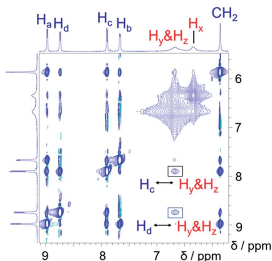
Fig. 6 ^1\text{H} - ^1\text{H} NOESY spectrum of a 1 : 6 mixture of \text{AzaEx}^2\text{Cage} \cdot 6\text{Cl} and \text{BH4EN} (500 MHz, \text{D}_2\text{O} , 298 K). Through-space proton couplings between the \text{H}_c and \text{H}_d protons in the phenylene groups of the cage and the \text{H}_y and/or \text{H}_z protons in the guests are labeled in the spectrum, demonstrating that \text{BH4EN} \cdot \text{AzaEx}^2\text{Cage}^{6+} may exist in the form of an inclusion complex in water.
